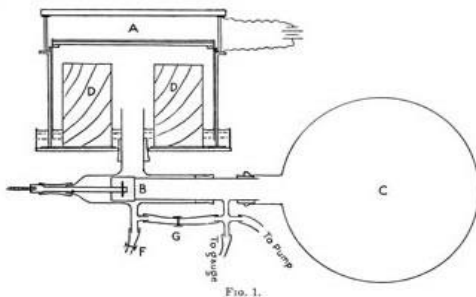
FIG. 1. A diagram of Wilson's apparatus. The cylindrical cloud chamber ('A') is 16.5cm across by 3.4cm deep.
