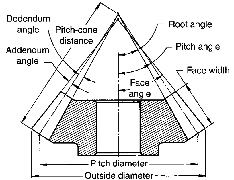
Fig. 14 Angles and terminology for straight bevel gears
