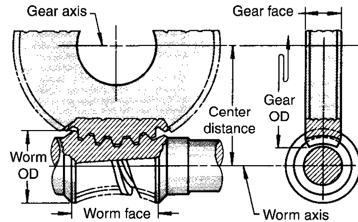
Fig. 16 Mating of worm gear (worm wheel) and worm in a double-enveloping worm gear set
