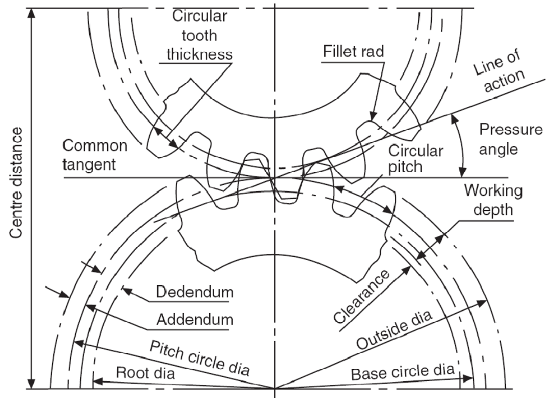
Fig. 24.15 Spur-gear terms
