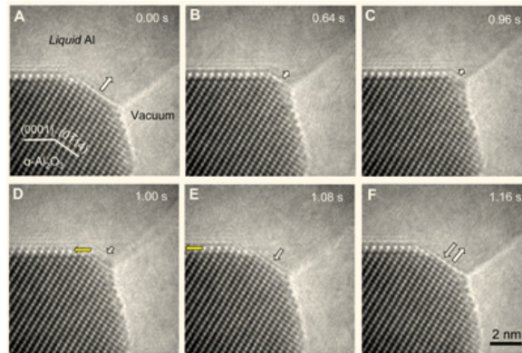
A sapphire nanowire's oscillatory growth
