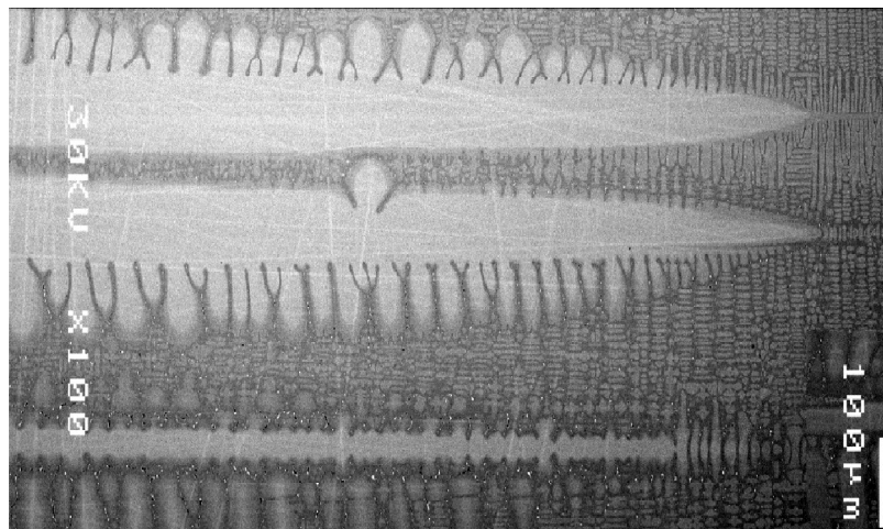
Non-faceted dendrites in a Ni super alloy
