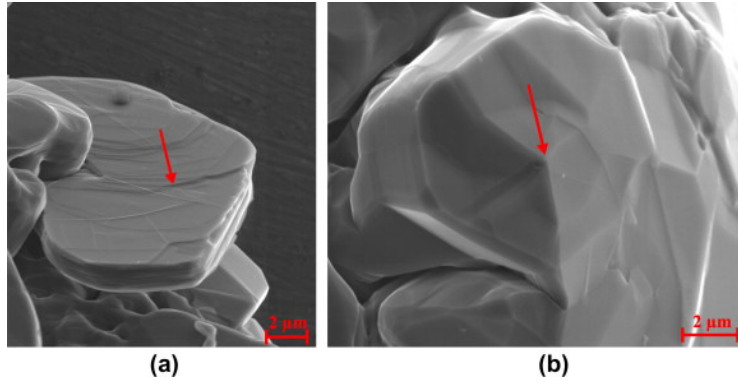
Faceted growth of graphite basal plane by (a) 2-D nucleation and migration of ledges and (b) spiral growth
