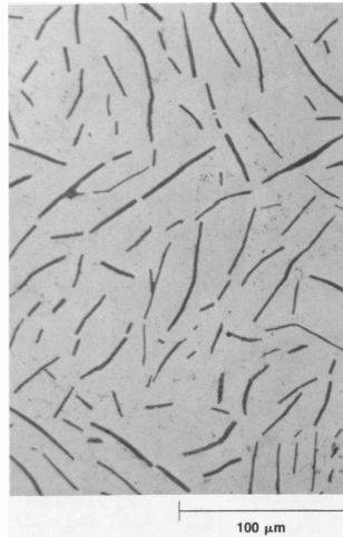
Graphite flake in Cast Iron
