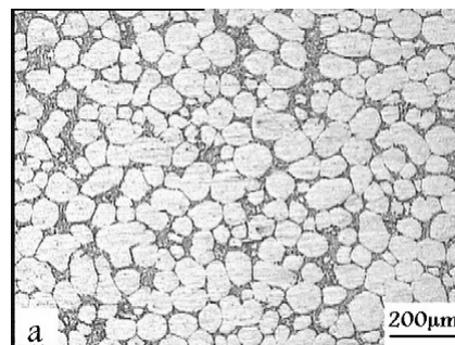
Non-faceted non-dendritic growth of a hypoeutectic Al-Si alloy
