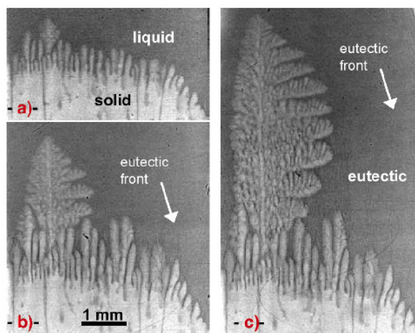
Non-faceted growth of dendrites in an Al-3.5Ni alloy
