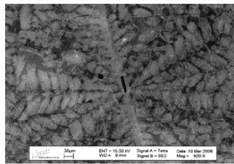
Figure 4. Dendrites presence in as-deposited microstructure (a). Detail of dendrites from white box region (b).
