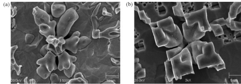
(a) Non-faceted and (b) non-faceted/faceted interfaces corresponding to primary VC
