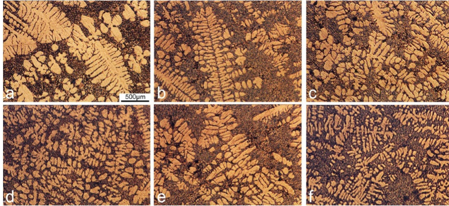
Fig. 1 - Effect of external pressure on the microstructure of squeeze cast LM13 alloy: (a) 0 (atmospheric pressure), (b) 20 MPa, (c) 53 MPa, (d) 106 MPa, (e) 171 MPa, (f) 211 MPa ( T_m = 730^\circ\text{C} and T_d = 200^\circ\text{C} ).
