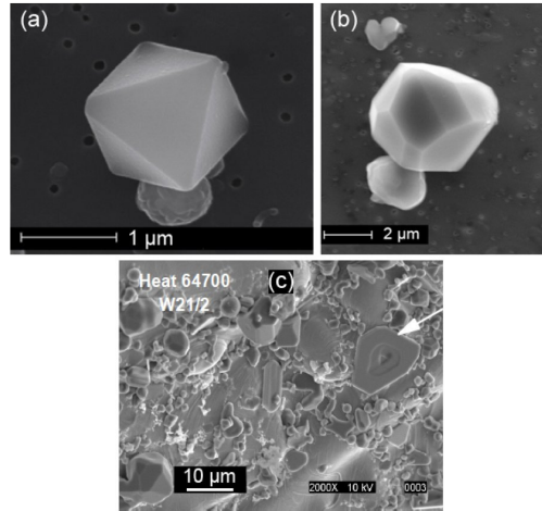
Faceted Al 2 O 3 inclusion (a) octahedral, (b) non-octahedral and (c) hopper morphologies (indicated by the arrow)
