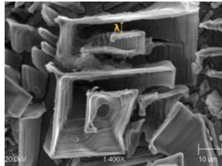
SEM micrograph of an eutectic Fe-C-V-Si alloy showing overlapping of VC x carbide spiral segments
