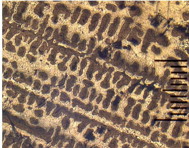
Non-faceted dendrites in a Pb-Sn solder
