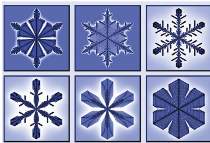
Faceted snowflake
