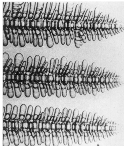
Non-faceted growth of SCN dendrites
