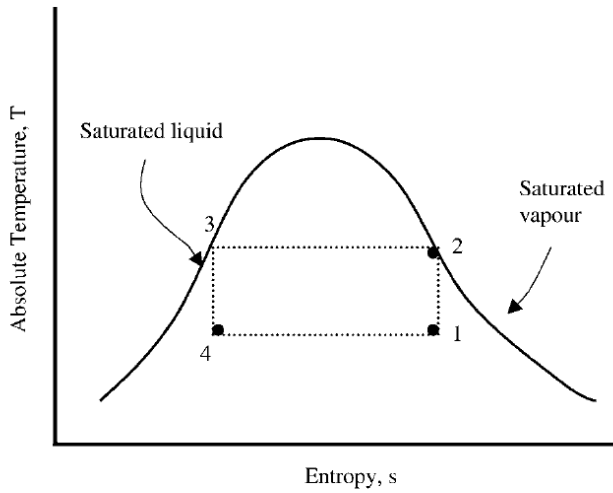
Fig. 4.3 Temperature-entropy diagram of the Carnot cycle.
