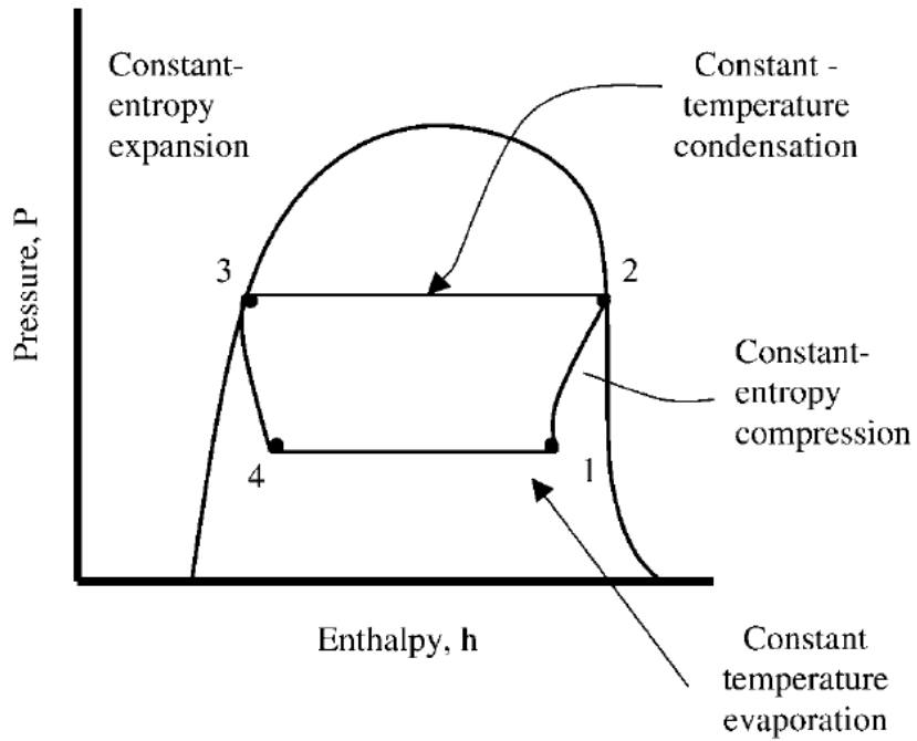
Fig. 4.2 Pressure-enthalpy diagram of the Carnot cycle.
