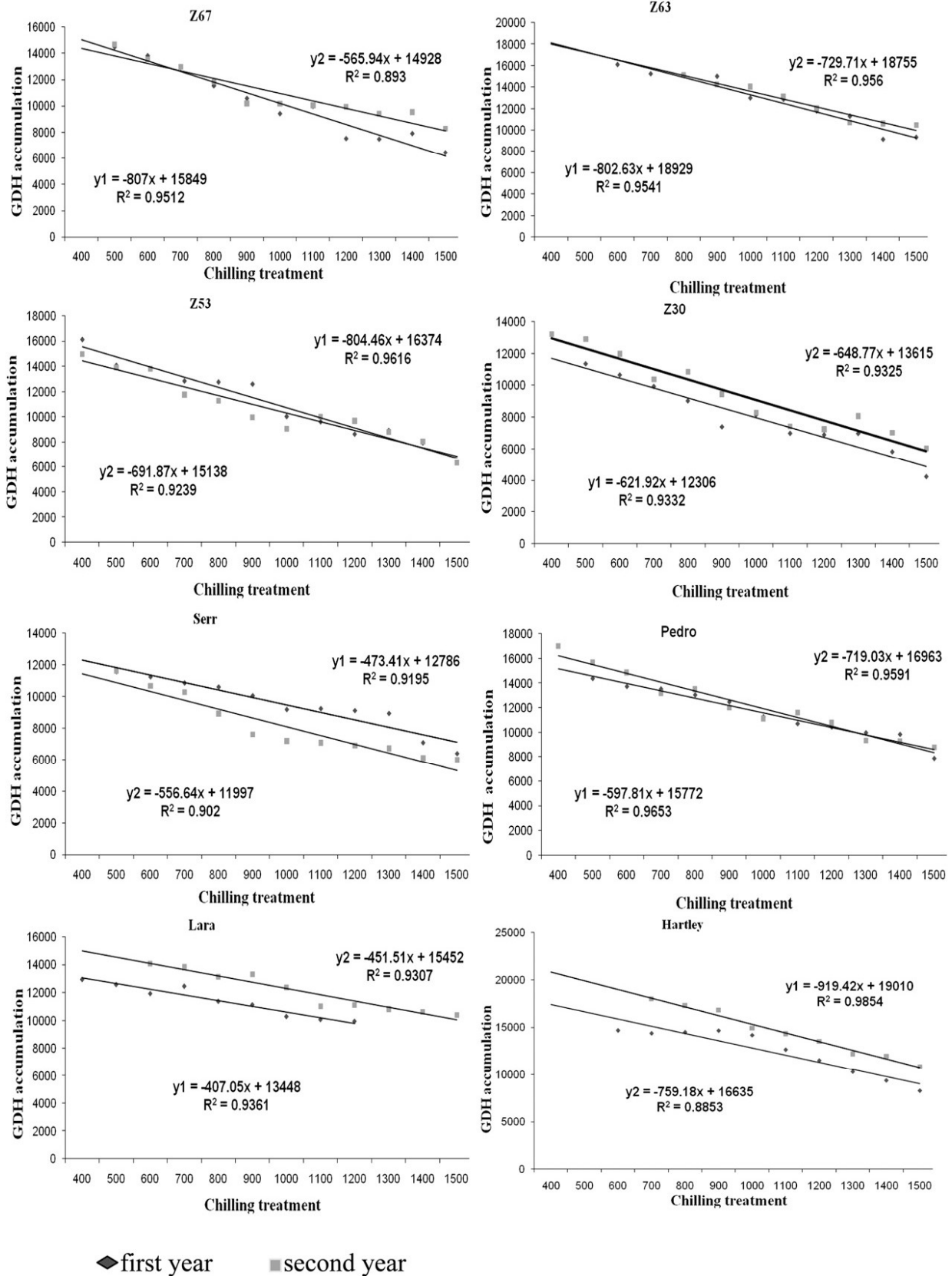
Fig. 1. The correlation between mean heat requirement and chilling treatments for all types of buds and catkin of Persian walnut cultivars and genotypes in 2 successive years along with the regression functions and coefficient of determination. Detached (or excised) twigs exposed to various chilling temperatures from 400 to 1500 and were forced to grow at 20 °C. The growing degree hours (GDH; °C) was calculated by the difference of 20 from 4.5 °C in 2 years.
