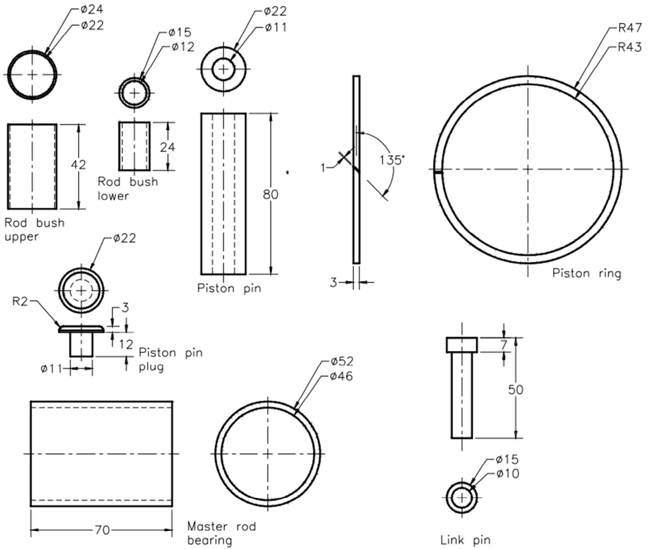
Figure 6 Views and dimensions of the Rod Bush Upper, Rod Bush Lower, Piston Pin Plug, Piston Pin, Piston Rings, and Master Rod Bearing
