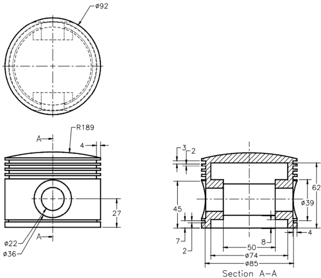
Figure 3 Views and dimensions of the Piston
