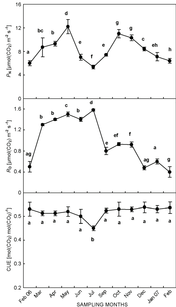
Fig. 1. Net photosynthetic rate ( P_N ), dark respiration rate ( R_D ), and carbon use efficiency (CUE) trend of Q. ilex during the study period. Standard error is shown. Monthly mean values with the same letters are not significantly different (ANOVA, p > 0.05 ).
