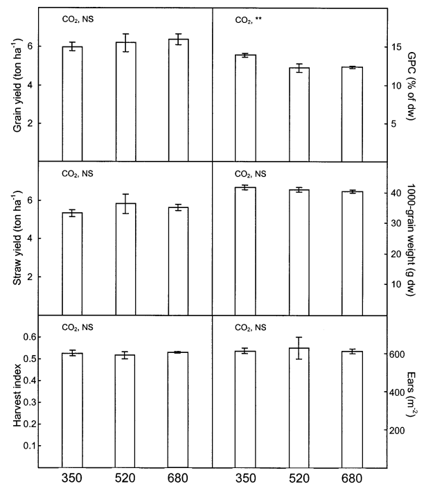
Fig. 3. Grain yield ( \text{ton ha}^{-1} ), grain protein concentration (GPC, %), straw yield ( \text{ton ha}^{-1} ), 1000-grain weight (g dry weight), harvest index and number of ears per square metre in the 1995 experiment. 350: 350 \mu\text{mol CO}_2 \text{ mol}^{-1} ; 520: 520 \mu\text{mol CO}_2 \text{ mol}^{-1} ; 680: 680 \mu\text{mol CO}_2 \text{ mol}^{-1} . Error bars show SE and the levels of significance are the results of a two-way ANOVA; NS: no significant treatment effect; significance level: ** P = 0.01 .
