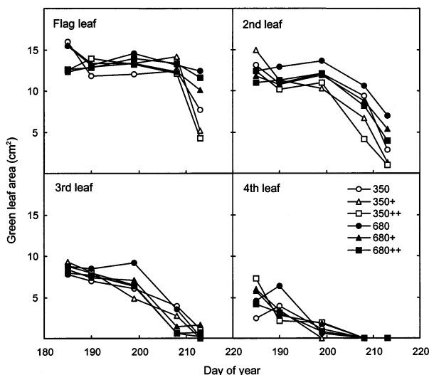
Fig. 5. Development of green leaf area per plant ( \text{cm}^2 ) for the youngest four leaves around and after anthesis in the different treatments in 1994. Mid-anthesis was at Julian day 190.
