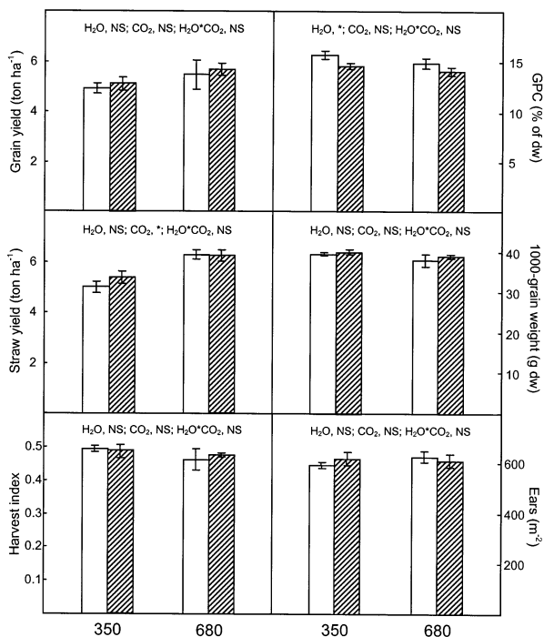
Fig. 4. Grain yield ( \text{ton ha}^{-1} ), grain protein concentration (GPC, %), straw yield ( \text{ton ha}^{-1} ), 1000-grain weight (g dry weight), harvest index and number of ears per square metre in the 1996 experiment. 350: 350 \mu\text{mol CO}_2 \text{ mol}^{-1} ; 680: 680 \mu\text{mol CO}_2 \text{ mol}^{-1} ; white bars: normal irrigation; hatched bars: increased irrigation. Error bars show SE and the levels of significance are the results of a two-way ANOVA; NS: no significant treatment effect; significance levels: * P = 0.05 .
